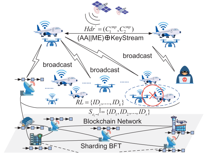
Fig. 2. Overview of our blockchain-based ADS-B secure BE scheme.
