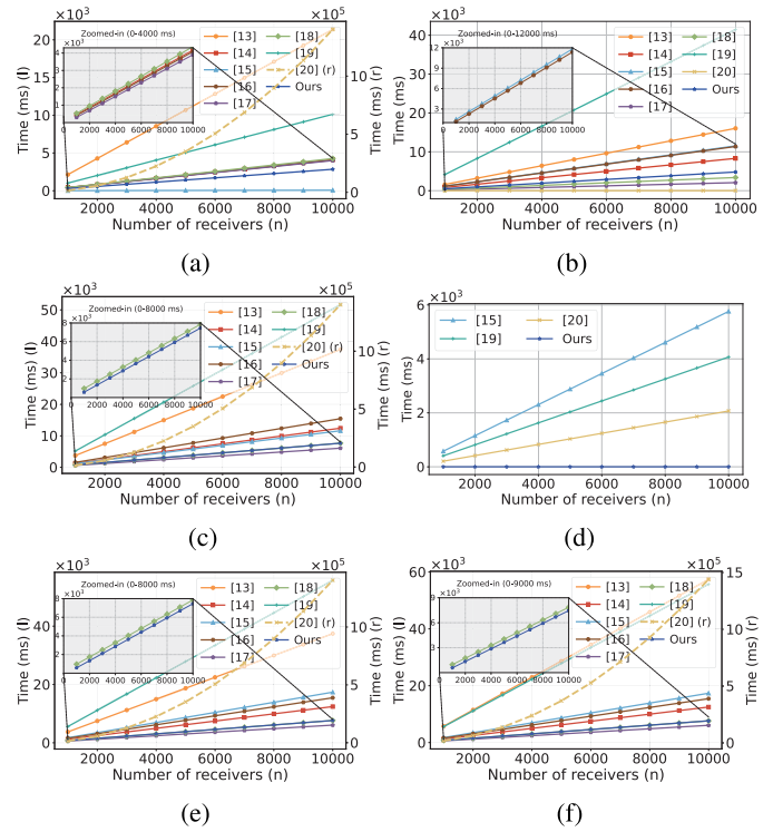
Fig. 8. Comparison of computation costs across different schemes for encryption, decryption, update/revocation, and message processing. (a) Encryption computation cost ( Hdr/K ). (b) Decryption computation cost ( Hdr/K ). (c) Total encryption and decryption cost ( Hdr/K ). (d) Update/revocation computation cost. (e) Total cost: encryption, decryption, and update/revocation ( Hdr/K ). (f) Final total computation cost: encryption and decryption of Hdr/K and message m .
